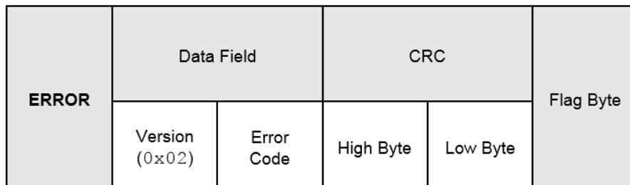
Figure 3.3. ERROR Frame Format
