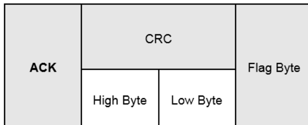
Figure 3.5. ACK Frame Format
